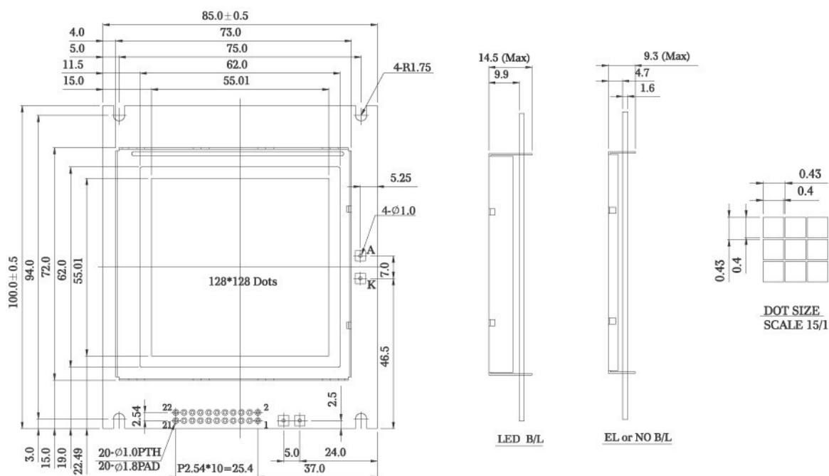
Dimension drawing
