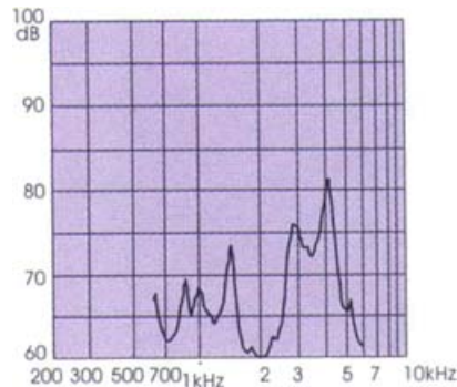
TFM-59DA-1 3V P-P Square Wave /10cm
