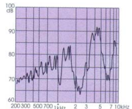
TFM-59DA-2 12V P-P Square Wave /10cm
