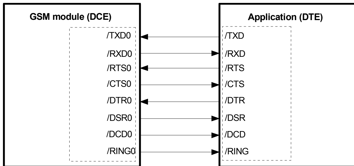
Figure 16: Serial interface
