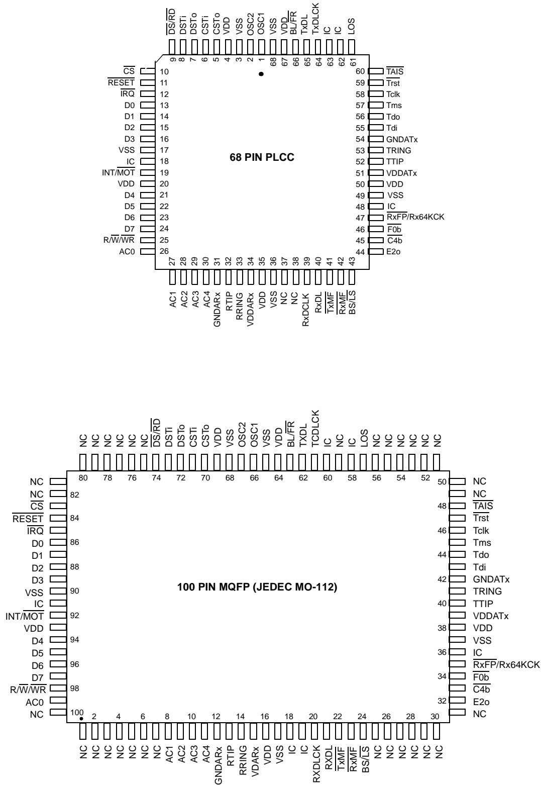
Figure 2 - Pin Connections
