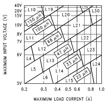
FIGURE 4. LM2598-3.3
