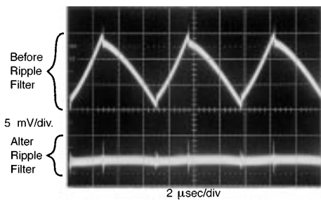
FIGURE 19. Post Ripple Filter Waveform
