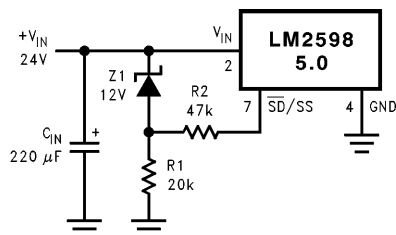
FIGURE 28. Undervoltage Lockout for a Buck Regulator
