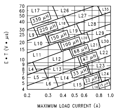
FIGURE 7. LM2598-ADJ
