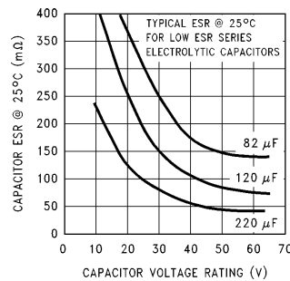
FIGURE 16. Capacitor ESR vs Capacitor Voltage Rating (Typical Low ESR Electrolytic Capacitor)
