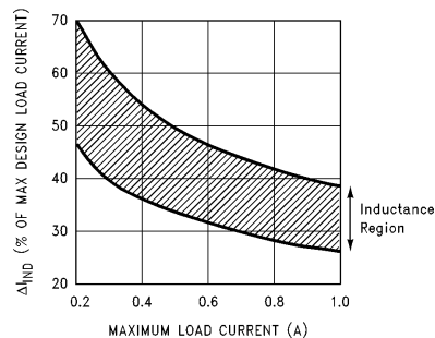
FIGURE 18. ( \Delta I_L / I_D ) Peak-to-Peak Inductor Ripple Current (as a Percentage of the Load Current) vs Load Current
