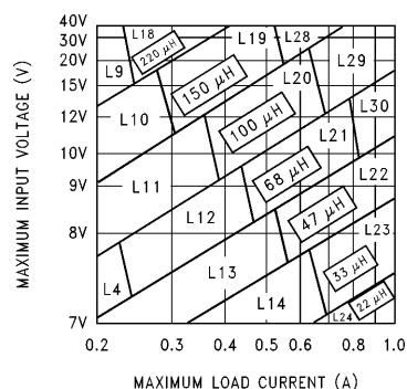
FIGURE 5. LM2598-5.0
