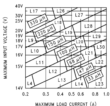
FIGURE 6. LM2598-12
