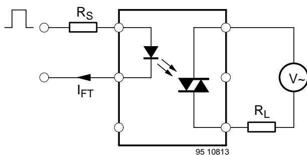
Figure 1. Test circuit for dv/dt_{\text{cr}} and dv/dt_{\text{crq}}
