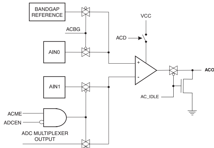
Figure 23-7. Analog Comparator
