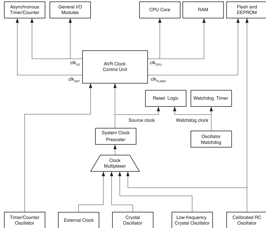
Figure 7-1. Clock Distribution
