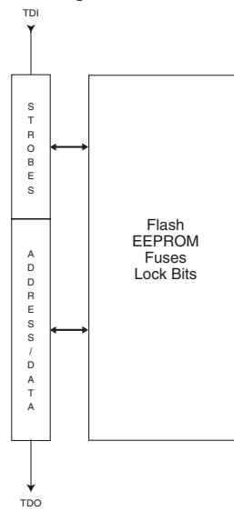
Figure 25-12. Programming Command Register
