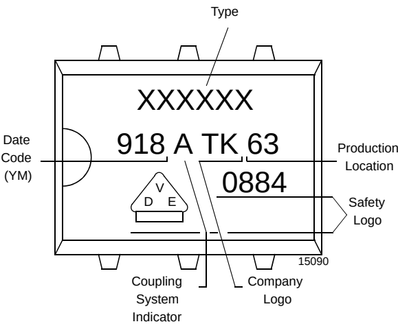
Figure 28. Marking example
