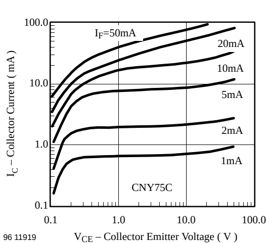
Figure 14. Collector Current vs. Collector Emitter Voltage
