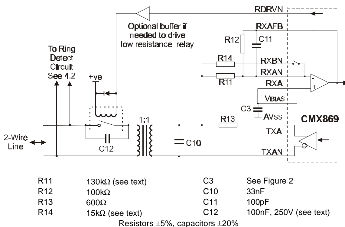
Figure 4a 2-Wire Line Interface Circuit
