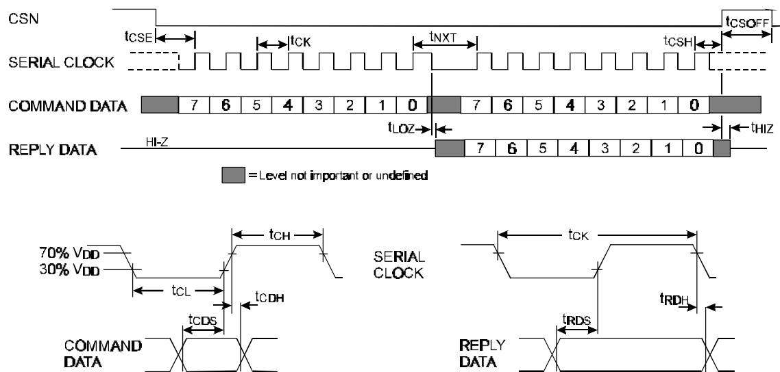
Figure 13 C-BUS Timing
