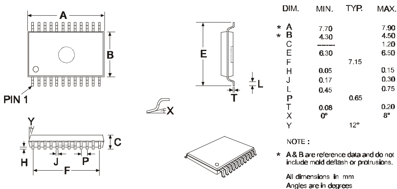
Figure 14b 24-pin TSSOP (E2) Mechanical Outline: Order as part no. CMX869E2
