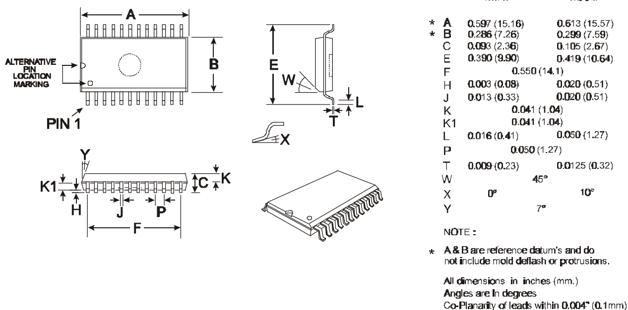
Figure 14a 24-pin SOIC (D2) Mechanical Outline: Order as part no. CMX869D2
