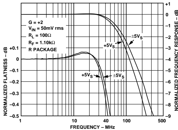
Figure 1. Frequency Response and Flatness, G = +2
