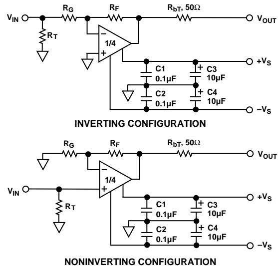
Figure 39. Inverting and Noninverting Configurations
