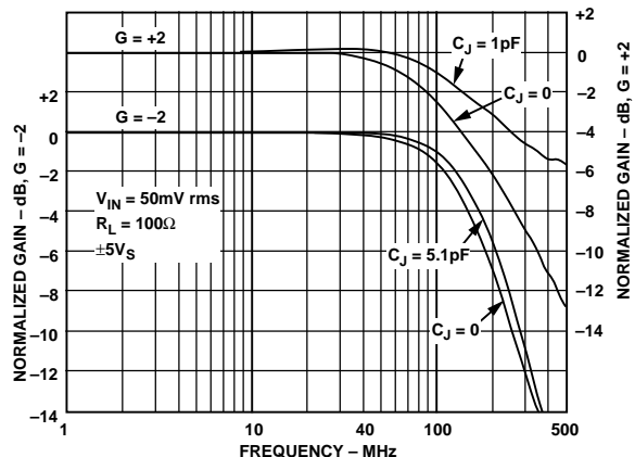
Figure 35. Frequency Response vs. Added Summing Junction Capacitance
