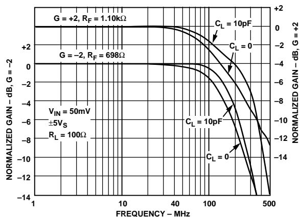
Figure 36. Frequency Response vs. Capacitive Loading, R_L = 100 \Omega Output
