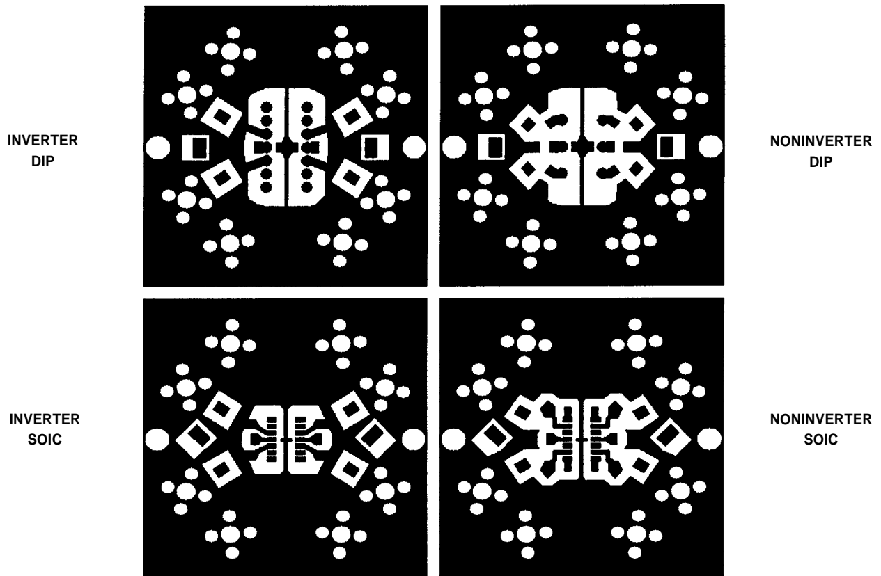
Figure 42. Evaluation Board Layout (Bottom Side, Looking Through the Board)
