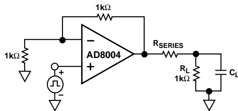
Figure 32. Driving Capacitive Load
