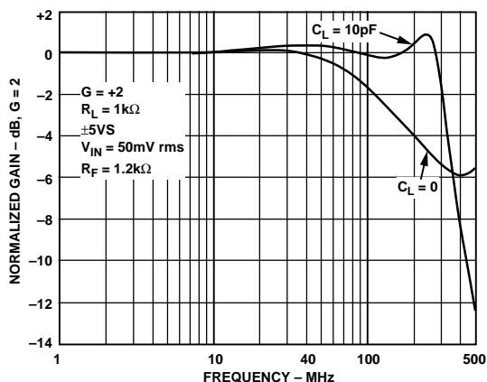
Figure 37. Flatness with 10 pF Capacitive Load
