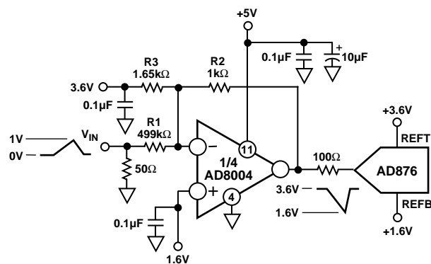
Figure 38. AD8004 Driving the AD876
