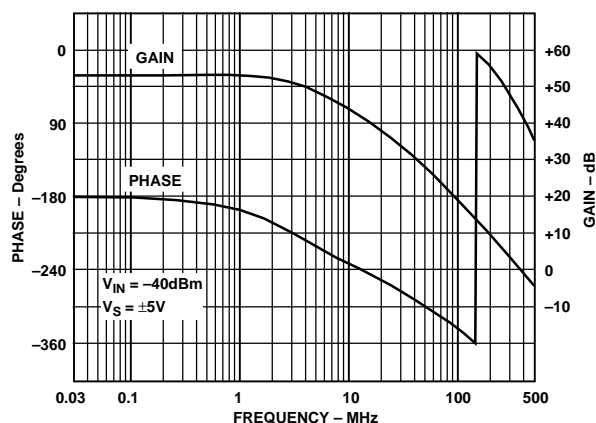
Figure 20. Open-Loop Voltage Gain and Phase
