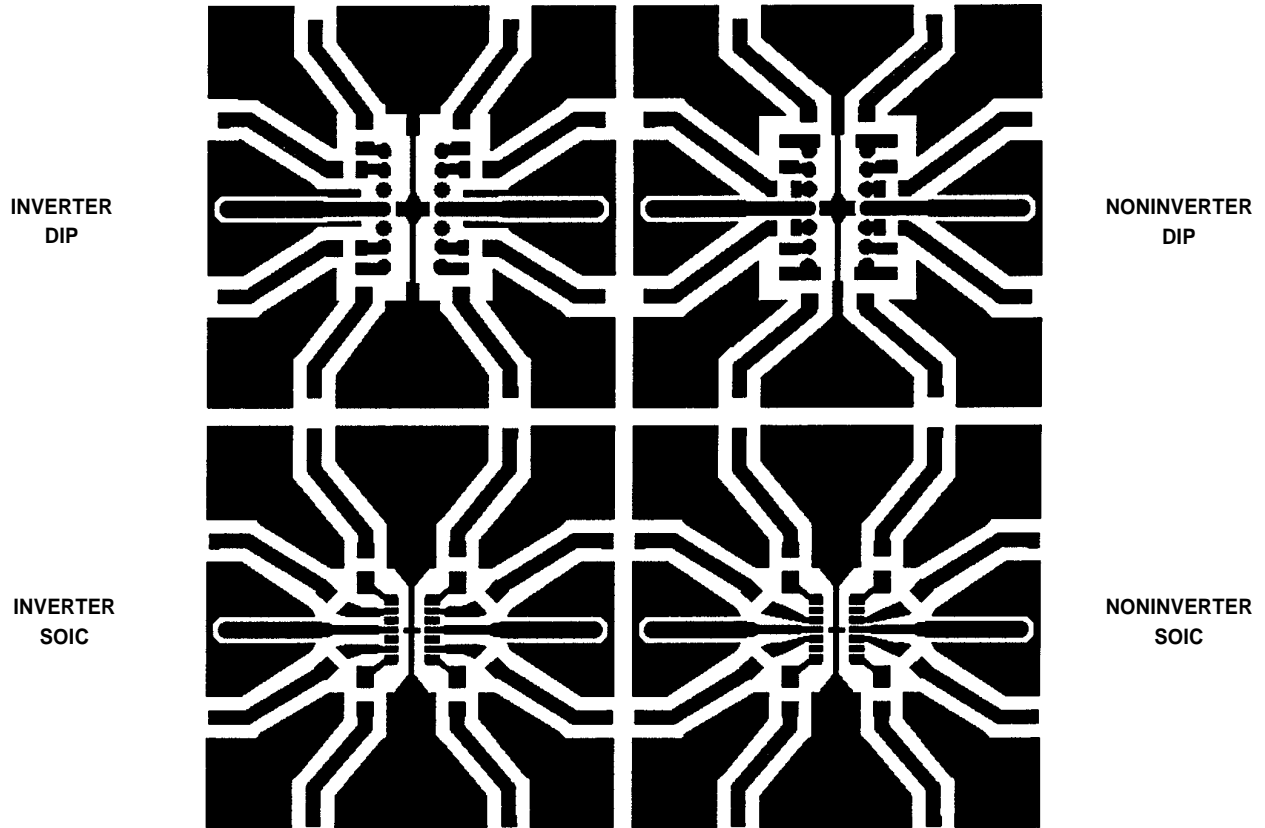
Figure 41. Evaluation Board Layout (Top Side)
