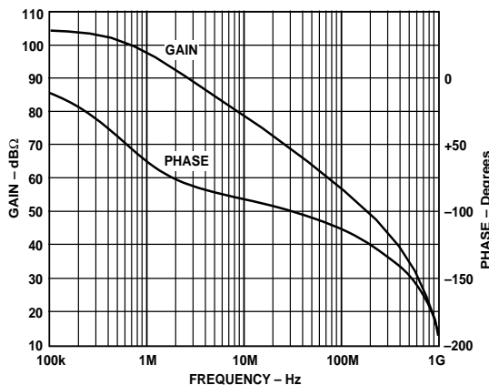
Figure 23. Open-Loop Transimpedance Gain
