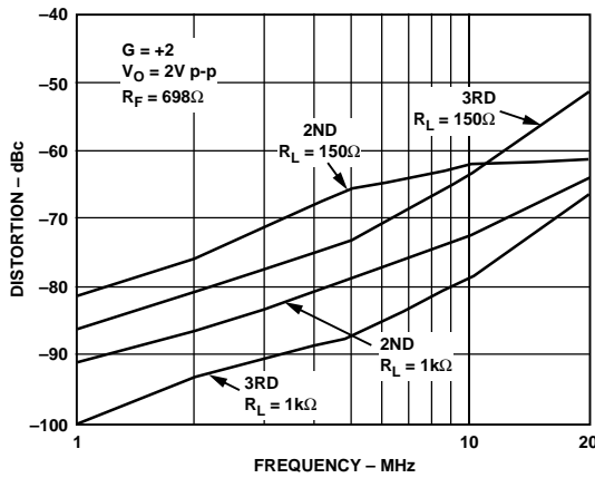
Figure 13. Distortion vs. Frequency; V_S = \pm 5\text{ V}
