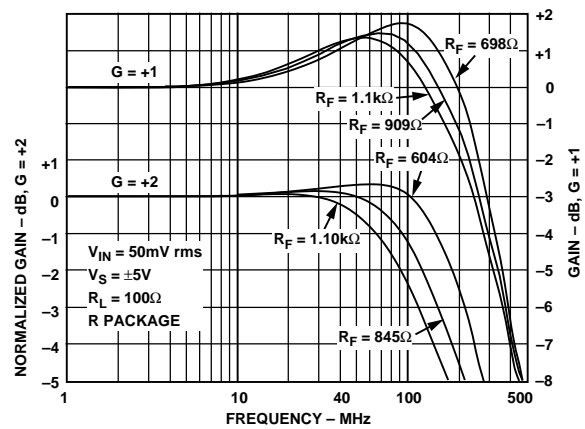
Figure 34. R_{FEEDBACK} vs. Frequency Response, G = +1/+2
