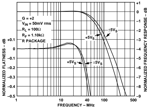
Figure 14. Frequency Response and Flatness, G = +2
