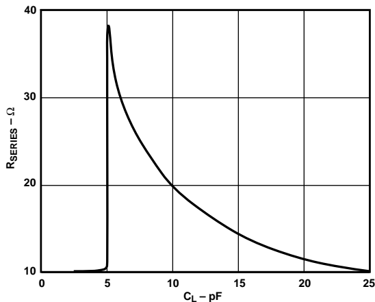
Figure 33. Recommended R_{SERIES} vs. Capacitive Load for \leq 30 ns Settling to 0.1%
