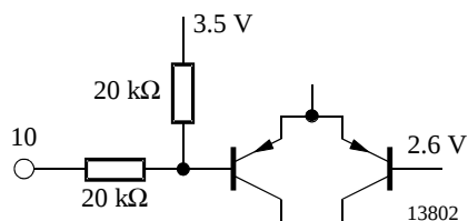
Figure 11. Mute switch (Pin 10)
