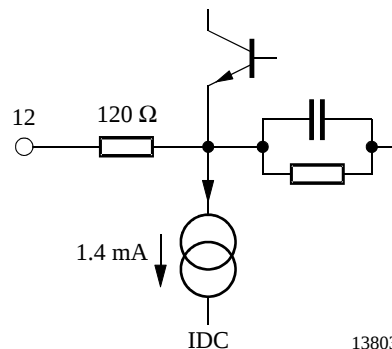
Figure 12. Inter-carrier output (Pin 12)
