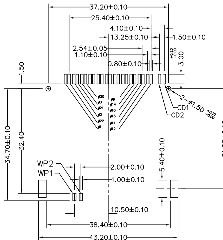
PCB Layout
