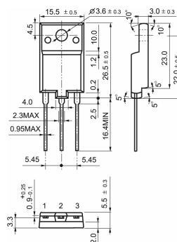
TO-3PM
