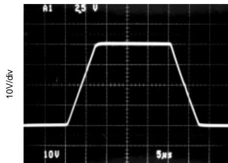
LARGE SIGNAL STEP RESPONSE G = 3, C_L = 100pF , R_L = 50\Omega
