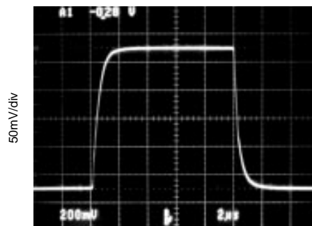
SMALL SIGNAL STEP RESPONSE G = 3, C_L = 1000pF
