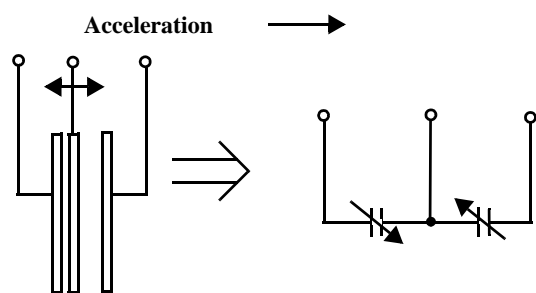
Figure 2. Simplified Transducer Physical Model
