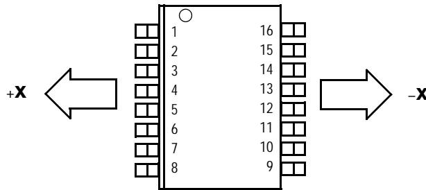
16-Pin SOIC Package
