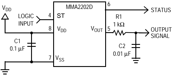
Figure 3. SOIC Accelerometer with Recommended Connection Diagram
