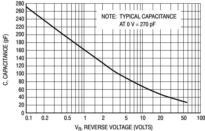
Figure 5. Typical Capacitance
