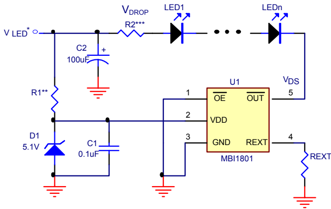
MBI1801 application circuit
