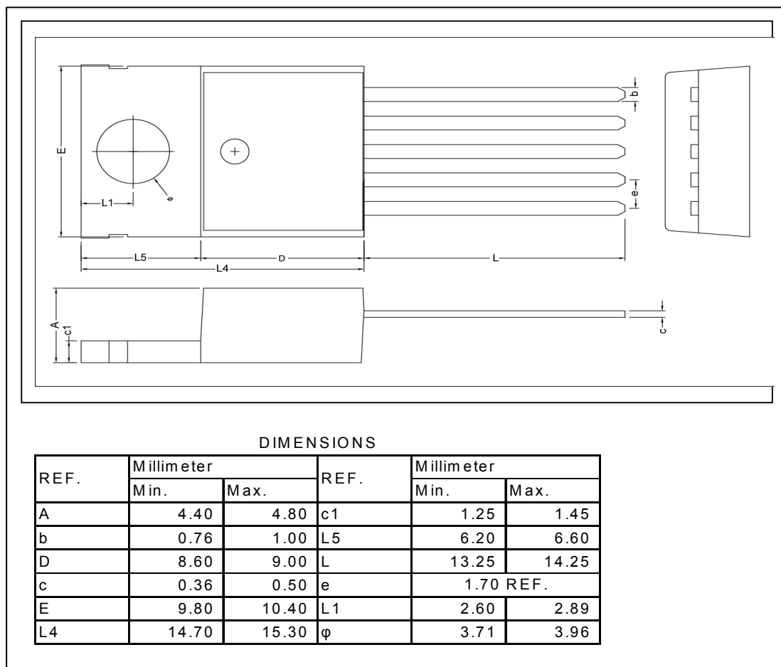
TO-220-5L
