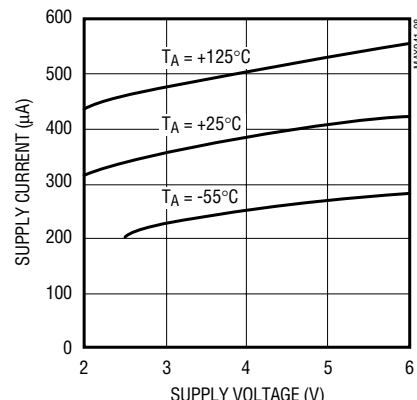
MAX941 TOTAL SUPPLY CURRENT vs. SUPPLY VOLTAGE
