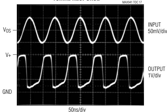
10MHz RESPONSE
