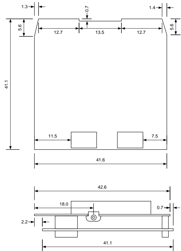
Digital Board
