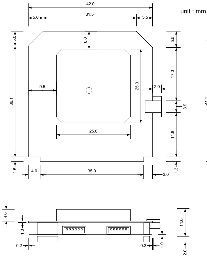
RF Board
