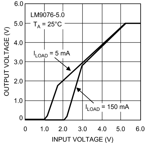
High Voltage Behavior
