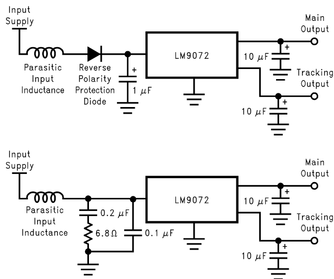
FIGURE 7. Input Bypassing
