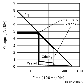
Turn-OFF Characteristic
