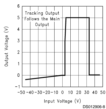
Main Output Voltage at Input Voltage Extremes
