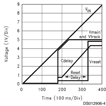
Turn-ON Characteristic
