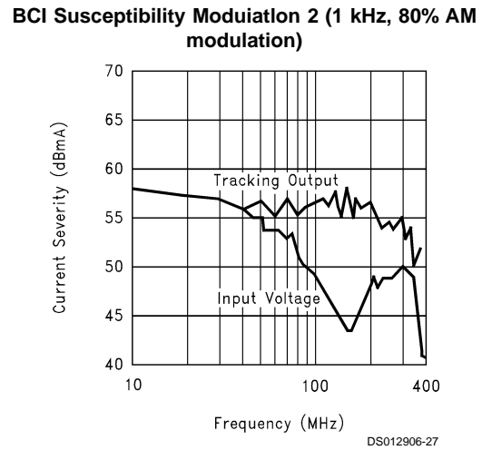
FIGURE 10. Examples of BCI Test Results
