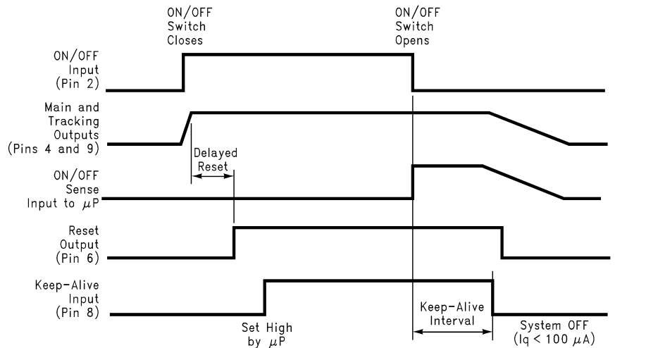
FIGURE 4. Basic Keep-Alive Operation
