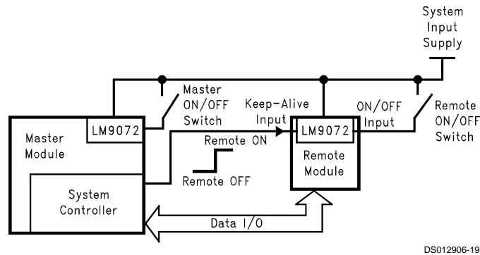
FIGURE 3. Remote ON/OFF Control
