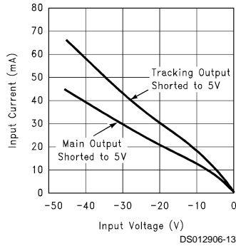
Reverse Battery Input Current
