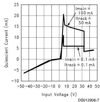
Quiescent Input Current vs Input Voltage
