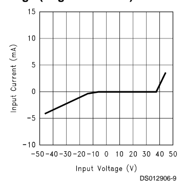
Input Current vs Input Voltage (Regulators OFF)
