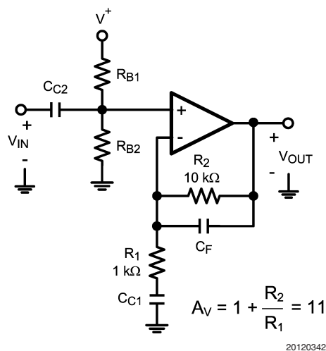
FIGURE 11. Non-Inverting Audio Preamplifier
