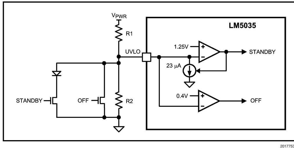
FIGURE 13. Remote Standby and Disable Control
