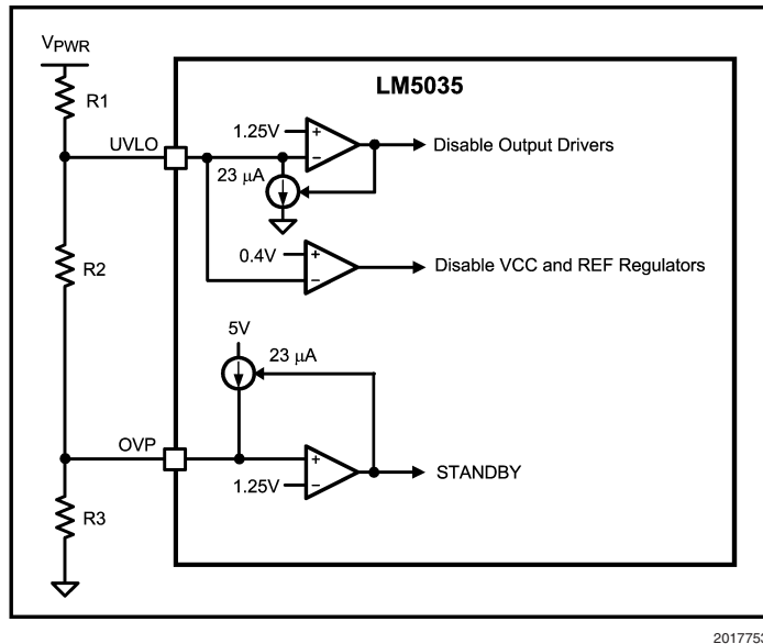
FIGURE 12. UVLO/OVP Divider
