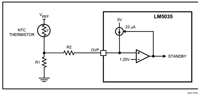
FIGURE 15. Remote Thermal Protection
