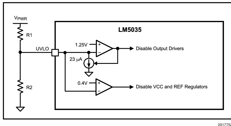
FIGURE 10. Basic UVLO Configuration
