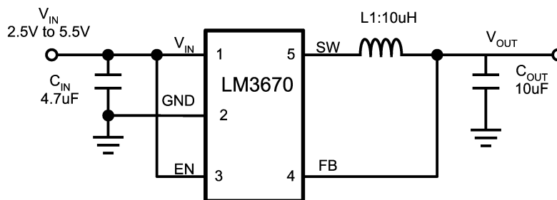
FIGURE 1. 1.8V - Fixed Output Voltage - Typical Application Circuit
