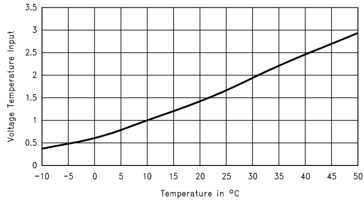
Typical Configuration Curve, (NTC Characteristics: 3 k \Omega @ 25°C, \beta=3988 )
