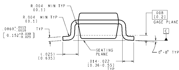
5-Lead SOT23-5 Package NS Package Number MF05A
