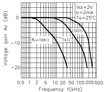
Fig. 10 Frequency Response
