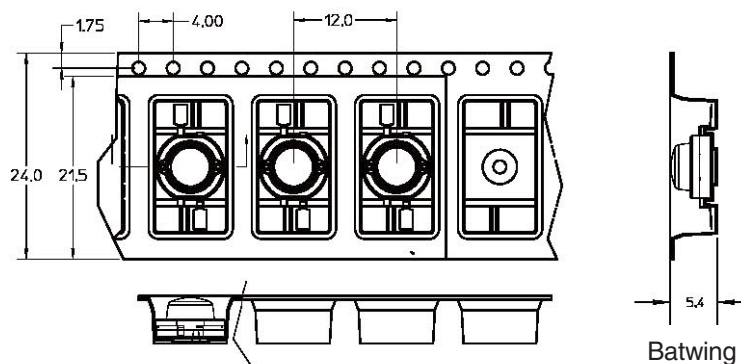
Figure 8. Tape dimensions for Batwing radiation pattern.
