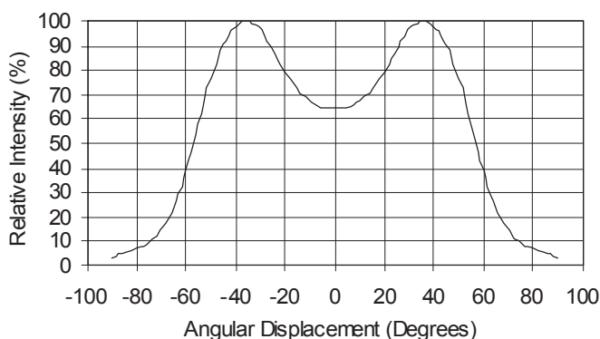
Figure 5. Typical Representative Spatial Radiation Pattern for LXHL-BW03 and LXHL-MWGC.
