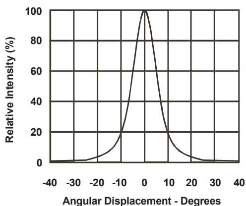
Figure 6. Typical Representative Spatial Radiation Pattern for LXHL-NWG8.
