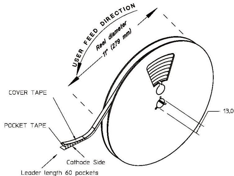
Figure 7. Reel dimensions and orientation.
