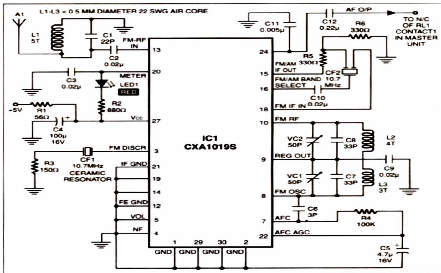
Circuit diagram of FM receiver using CXA1019S
