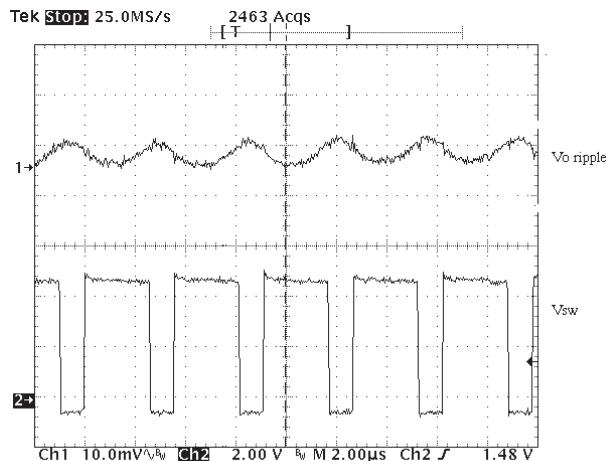
Figure 12. The Output Voltage Ripple Using Two 10 \mu\text{F} Ceramic Capacitors in Parallel
