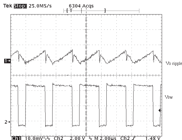
Figure 15. The Output Voltage Ripple Using One 100 \mu\text{F} Tantalum Capacitor
