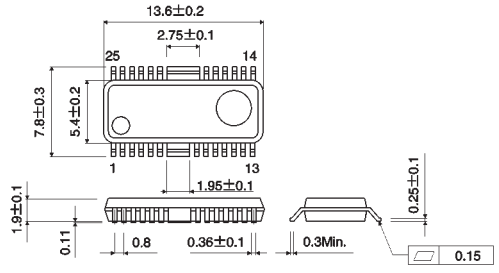
HSOP25
