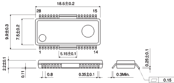
HSOP28
