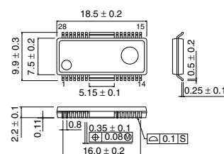
HSOP-M28
