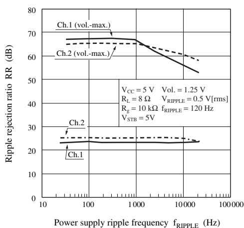
RR — f_{\text{RIPPLE}}
