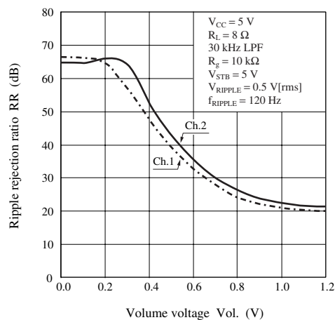
RR — Vol.
