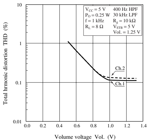
THD — Vol.
