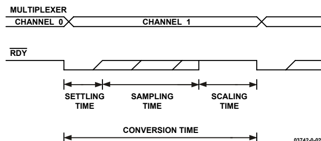
Figure 25. Multiplexer and Conversion Timing—Continuous Conversion on Several Channels with Chopping Disabled
