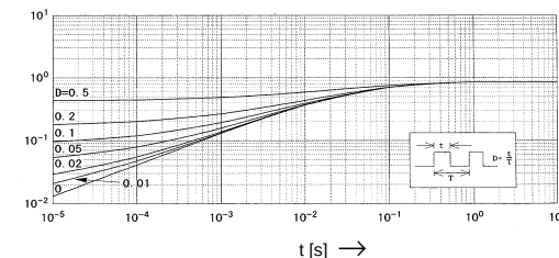
Z_{th(ch-e)} [K/W]
