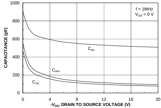
Figure 19. Capacitance Characteristics.
